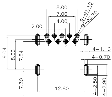
RECOMMENDED P.C.B LAYOUT(TOP VIEW) THICKNESS 1.60mm(TOLERANCE:±0.05)
